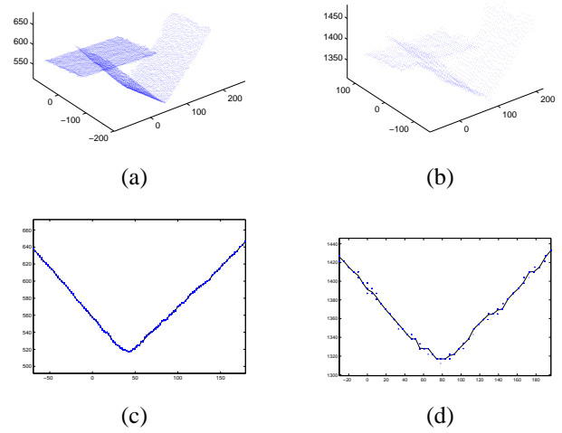
Fig. 2. Variations in the quality of captured depth: (a) and (b) are 3D scans of the same object, captured with the same depth sensor. (c) and (d) show cross section views of the same data. Clearly data in the left column is denser and less noisy.
