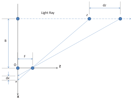
Fig. 3. Geometric relationships in a structured light setup.
