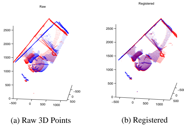
Fig. 1. Point cloud registration with ICP.
